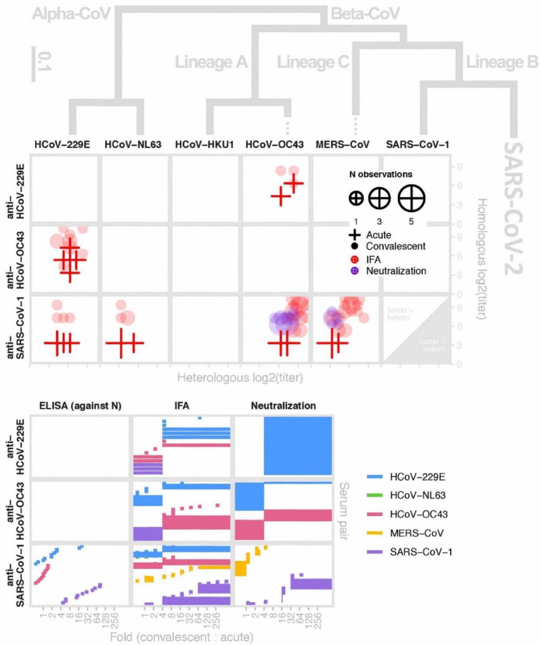
Figure 5: Antigenic and phylogenetic relationships among Human Coronavirus strains (Top) and Serological titers for comparison with confirmed infections of each virus (Bottom). The caption text is partially obscured and contains some errors. A clearer version of the caption is provided below.
