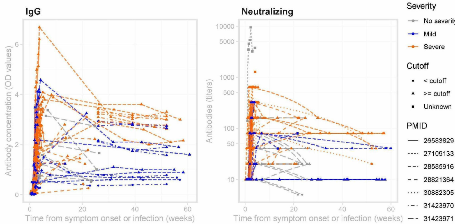
Figure 4: MERS-CoV antibody kinetics. The left panel shows data for studies reporting IgG concentration in units of optical density, while the right panel shows data for studies reporting neutralizing antibodies in units of titers. The plotting symbols indicate whether a measurement was above the cutoff for the assay being used, if reported in the study. Some studies reported titers that were lower than or greater than some threshold value; those are here plotted at those values (e.g., for \geq 320 , the value is assumed to be 320). Some studies may report kinetics of different antibodies or using different assays (and different units) for the same patient. Note that while these are plotted on the same axes, values may not necessarily be comparable across studies within each panel, as each lab may have different assay conditions resulting in different scales. See Figures S2 and S3 for (more limited) data on SARS-CoV-1 and IgA.
