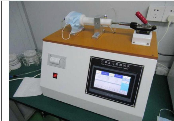
Differential pressure test
