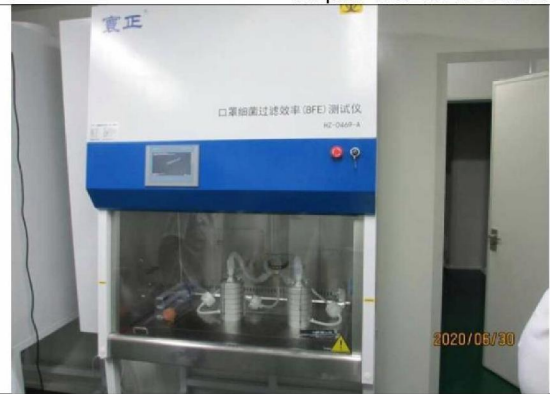
Bacterial filtration efficiency test
