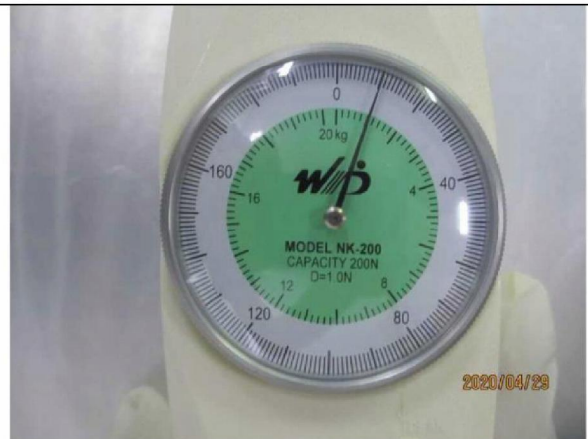
Ear strap strength test 1kgs weight(10N)
