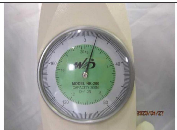
Ear strap strength test 1kgs weight 1minute, ok
